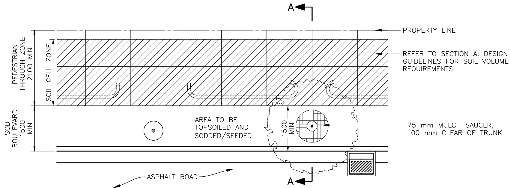
PLAN SCALE 1:75
