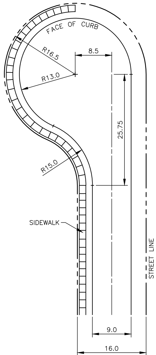
TYPE 2 LEFT OFFSET CUL-DE-SAC
